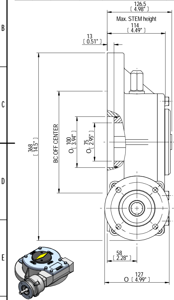
ISOMETRIC VIEW 1:10
