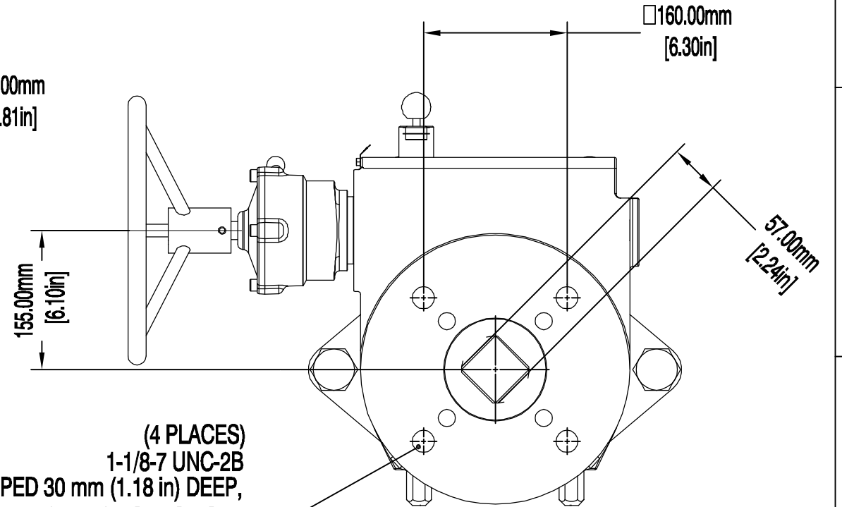
VALVE SIDE MOUNTING VIEW
