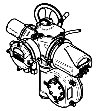
ISOMETRIC VIEW (SCALE 1:12)
