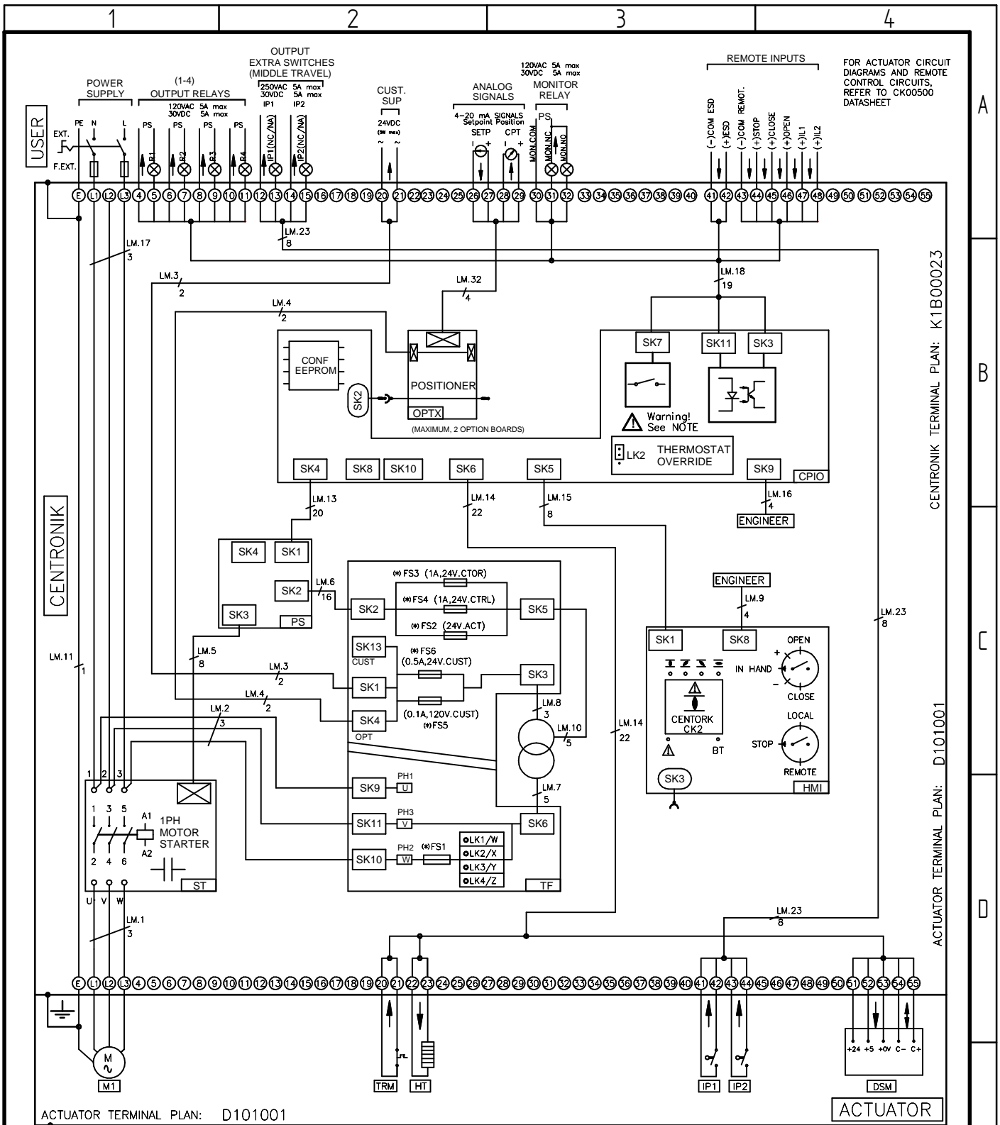
ACTUATOR TERMINAL PLAN: D101001
