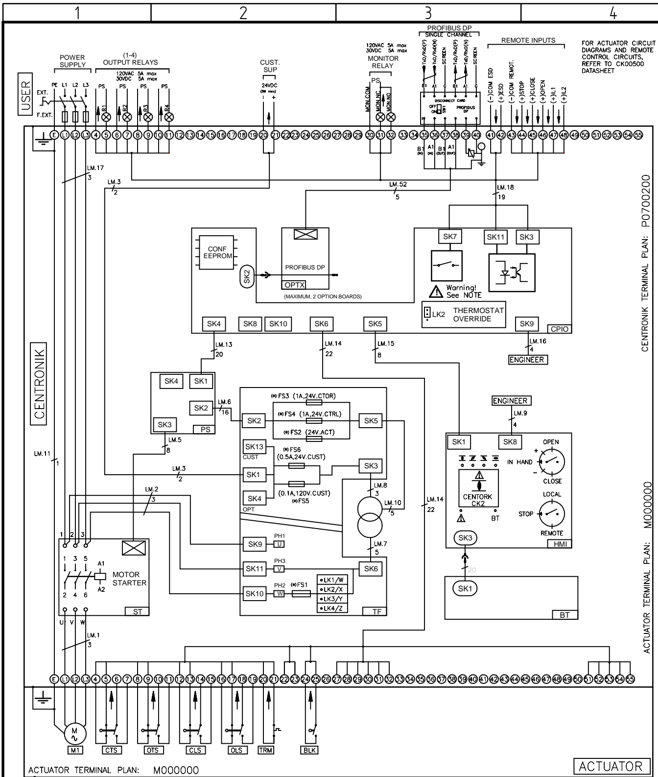
ACTUATOR TERMINAL PLAN: M000000
