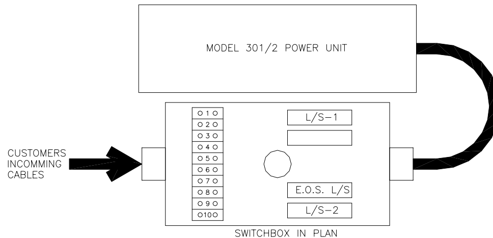
LIMIT SWITCHES SHOWN IN POSITION FOR ANTI-CLOCKWISE FAIL-SAFE
