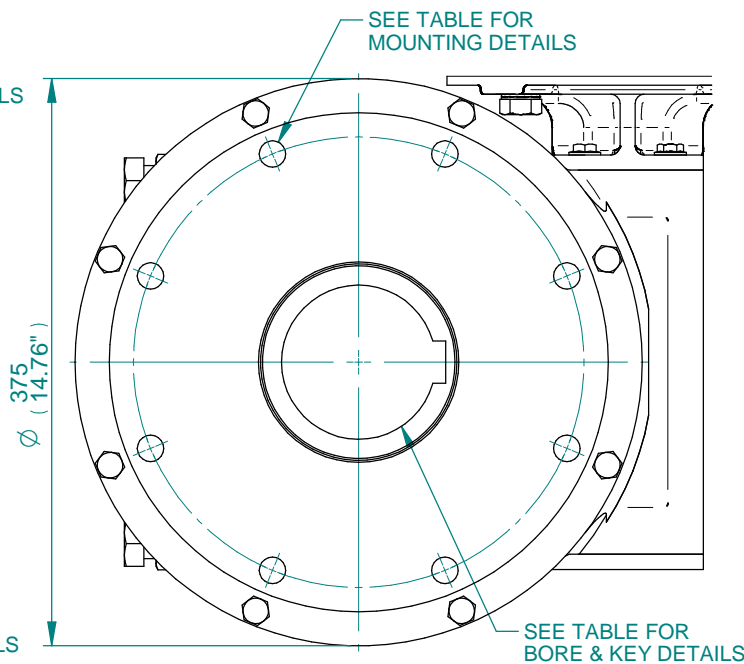
IW6 GEARBOX MOUNTING DETAILS FOR F25/FA25 & F30/FA30
