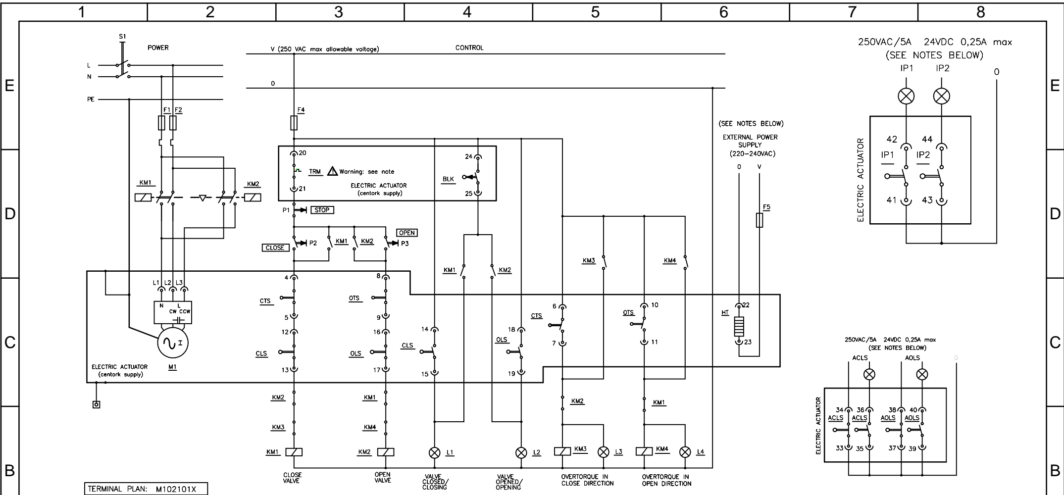
TERMINAL PLAN: M102101X
