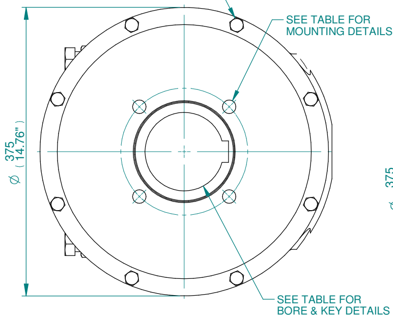
IW6 GEARBOX MOUNTING DETAILS FOR F16/FA16
