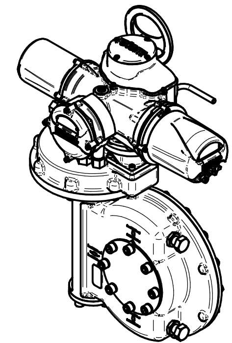
ISOMETRIC VIEW (SCALE 1:12)
