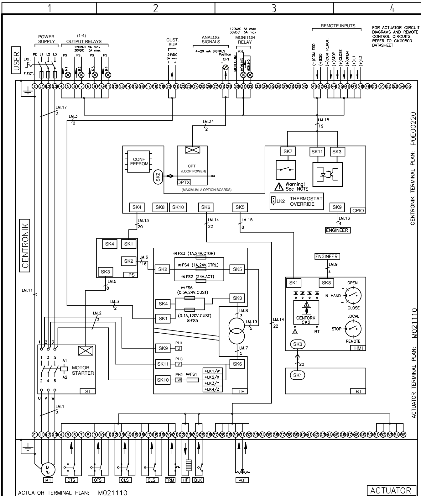
ACTUATOR TERMINAL PLAN: M021110
