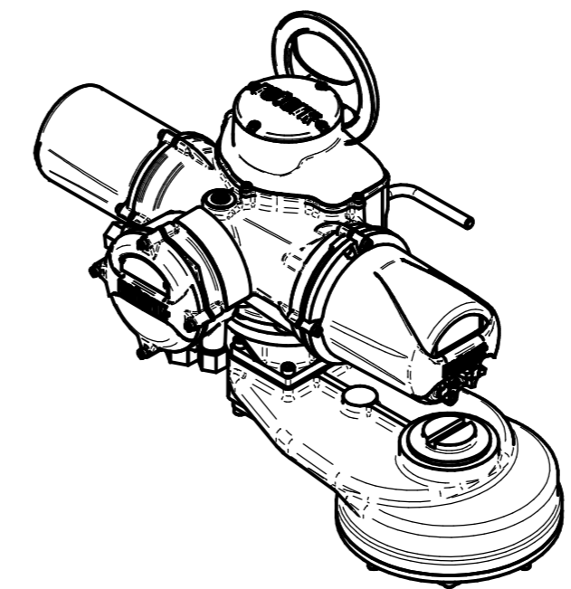
ISOMETRIC VIEW 1:10
