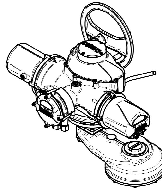
ISOMETRIC VIEW 1:10
