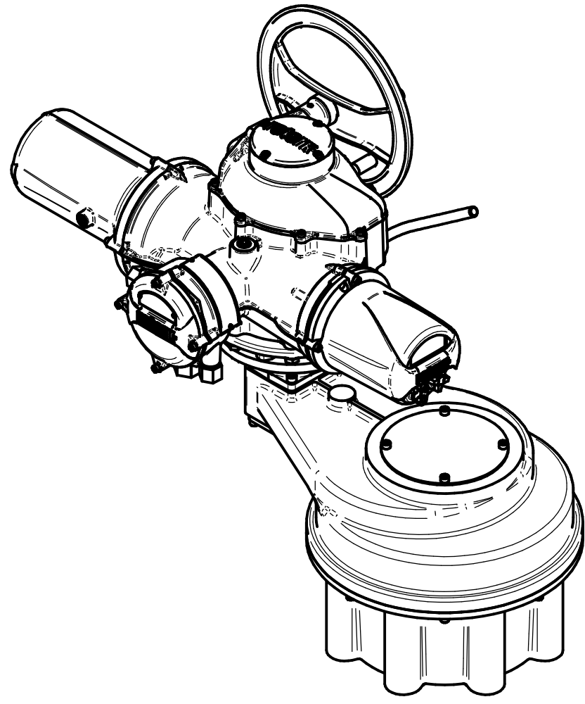
ISOMETRIC VIEW 1:10
