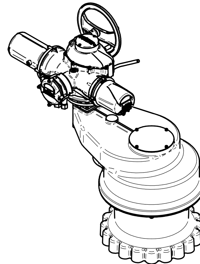
ISOMETRIC VIEW 1:15
