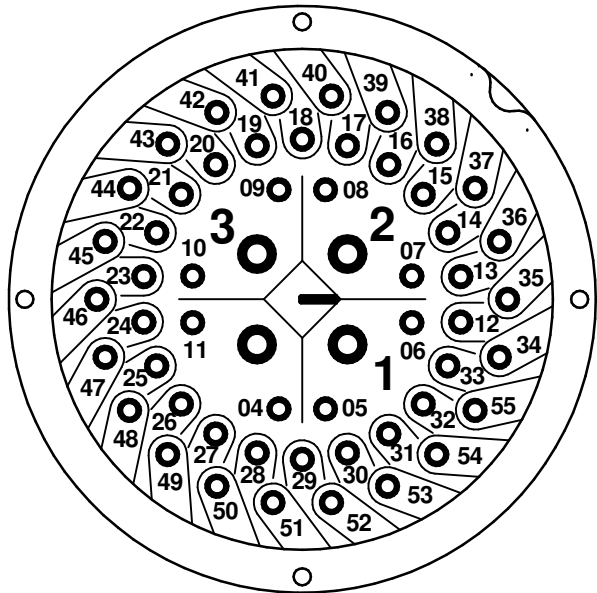
PLUG-AND-SOCKET CONNECTOR LAYOUT DISTRIBUCION CONECTOR PLUG AND SOCKET
