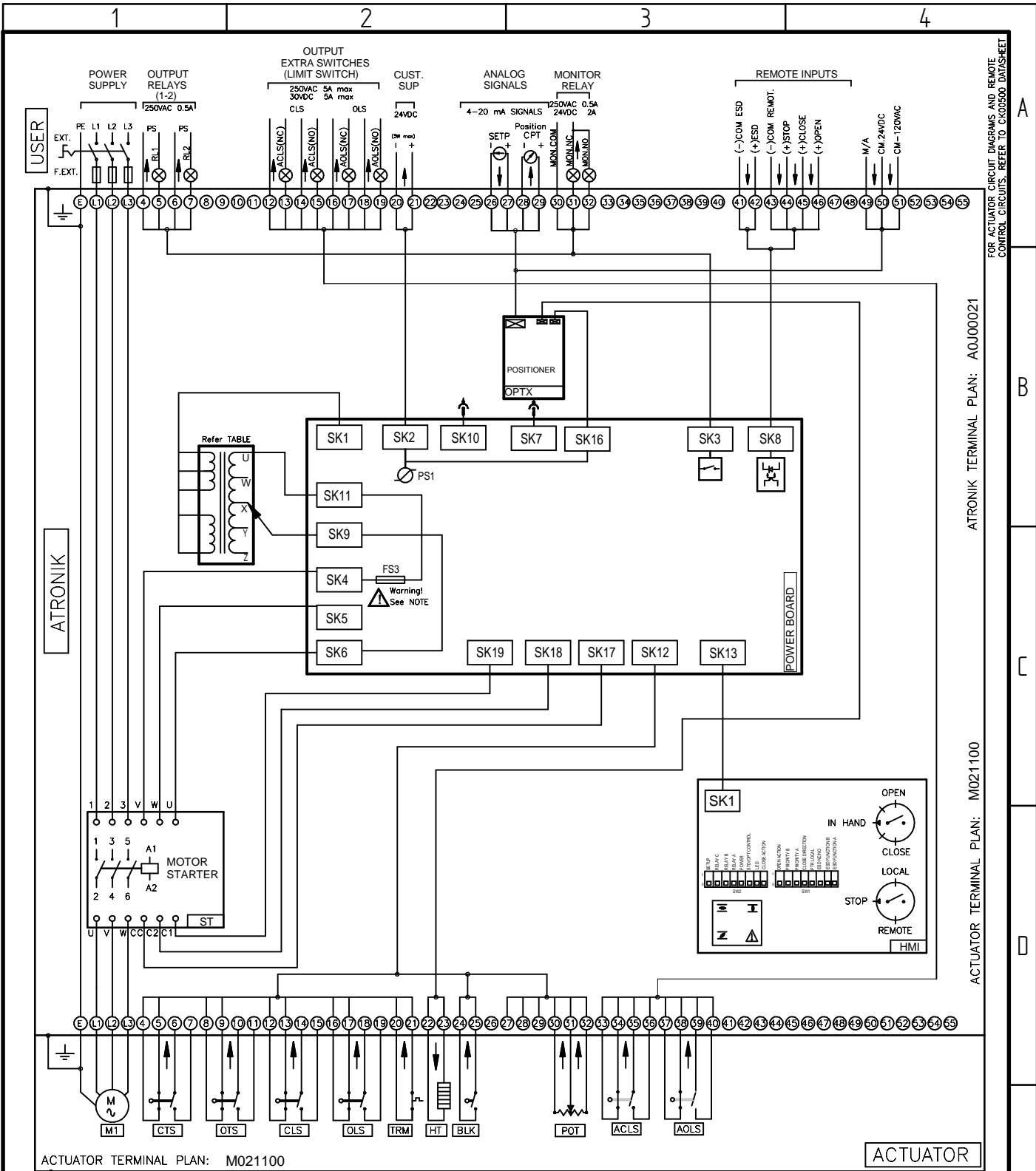
ACTUATOR TERMINAL PLAN: M021100
