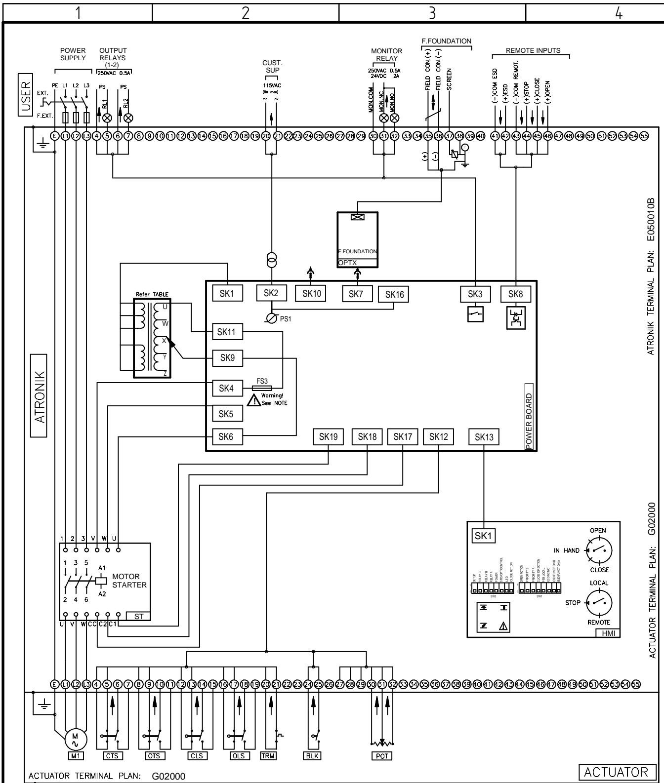
ACTUATOR TERMINAL PLAN: G02000
