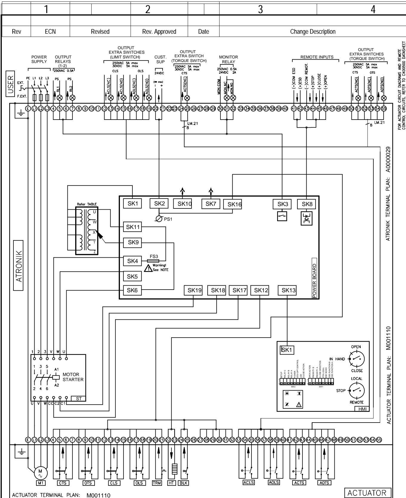
ACTUATOR TERMINAL PLAN: M001110
